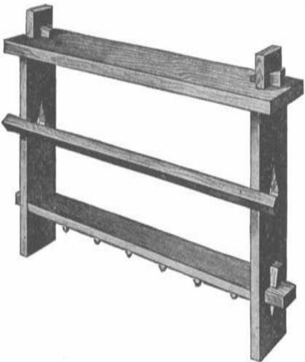
Parts Held Together by Keys
