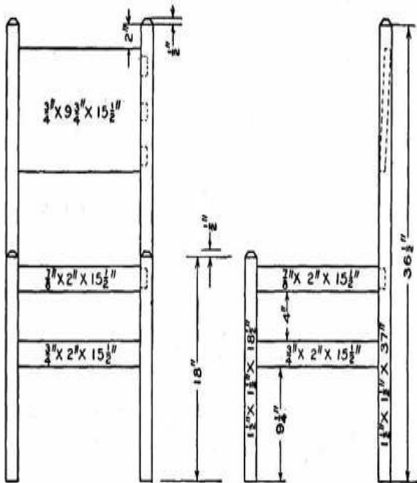
Details of Side Chair
