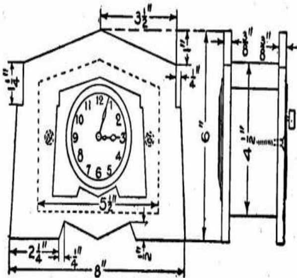
Details of Mantel Clock
