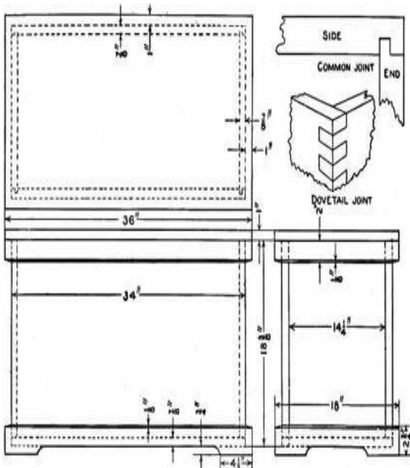
Details of Cedar Chest
