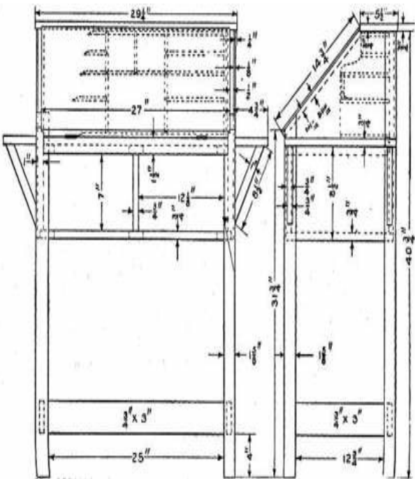
Detail of Writing Desk
