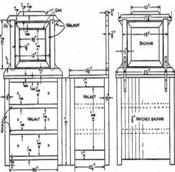
Details of Dresser
