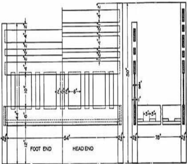
Details of Oak Bedstead
