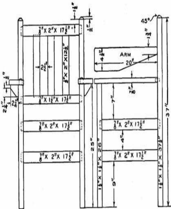
Details of Chair
