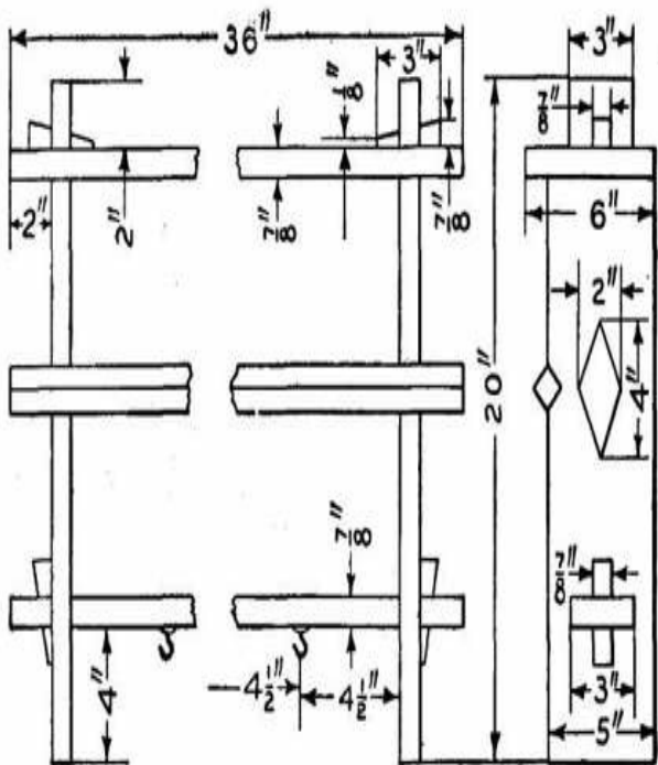
Details of Plate Rack
